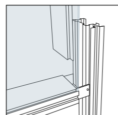
Telaio vetro. Glazed surface support profiles.
